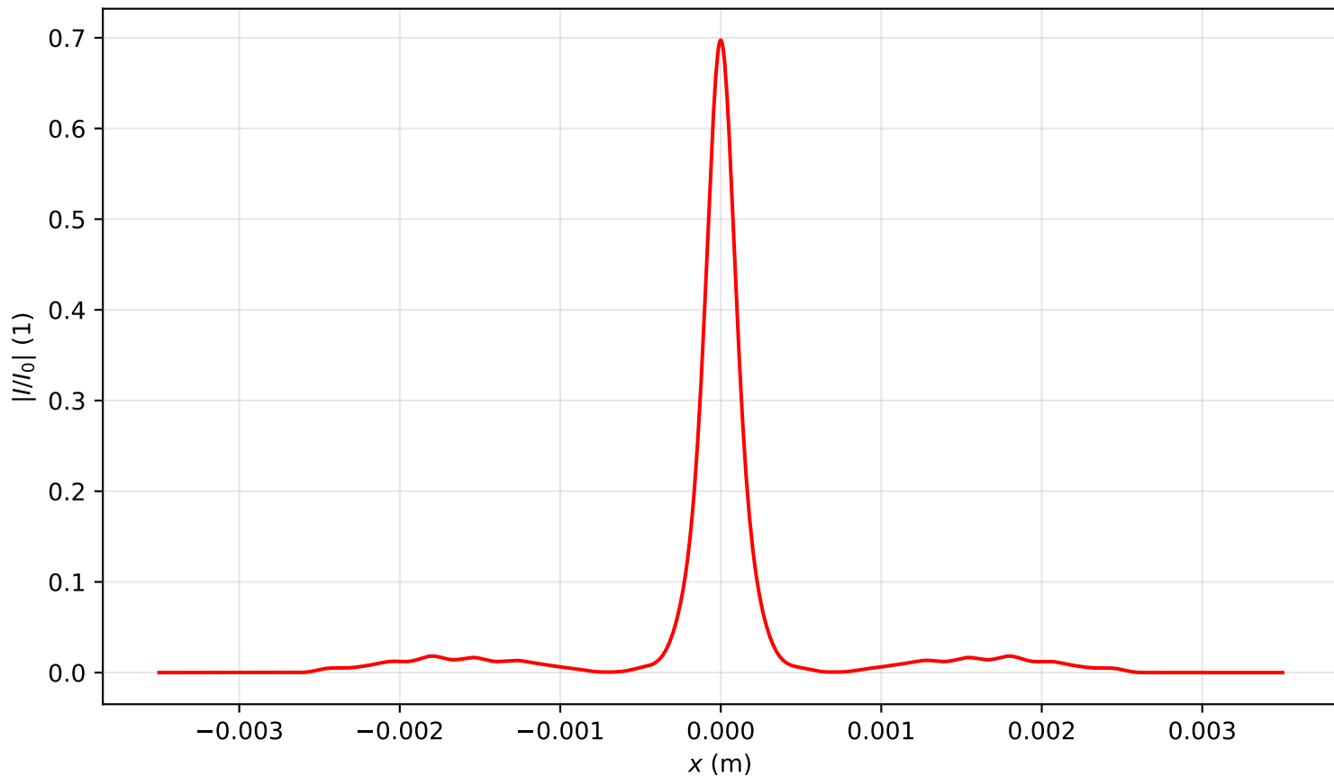
Intensity profile I(x, y = 0, z = 1.751)/I_0 , P_{in}=9.0P_{cr} , artificial time
